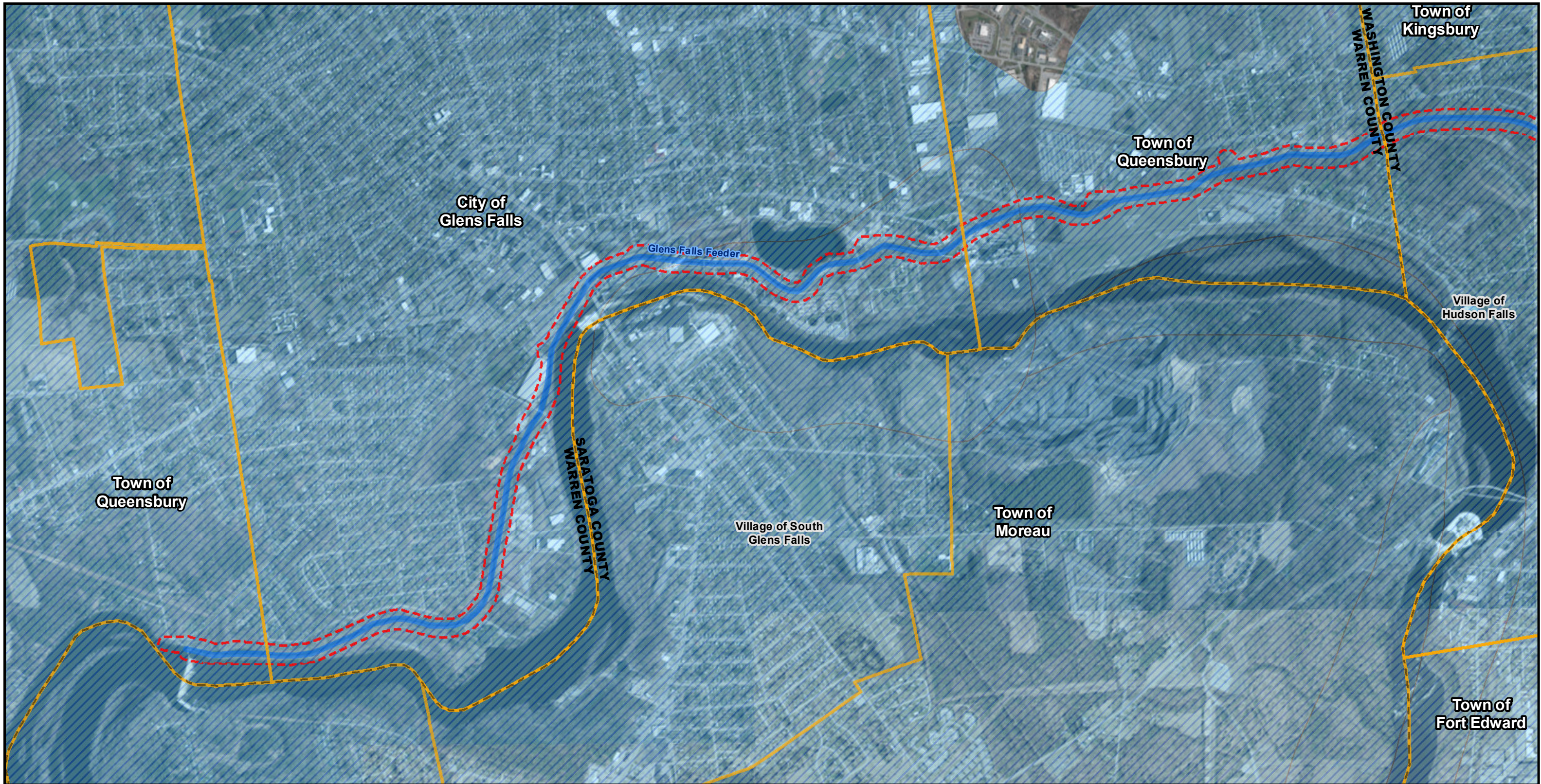
Figure 5F: Aquifers
